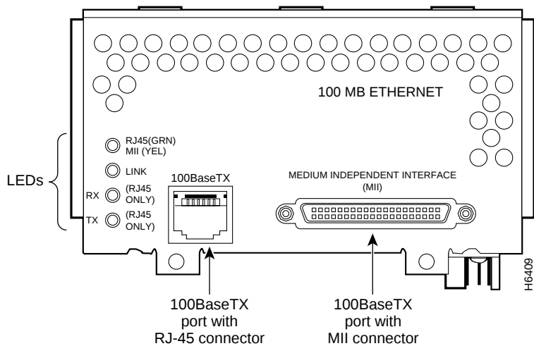
Figure 5-60: 1-Port 100BaseTX Fast Ethernet NPM (NP-1FE)
